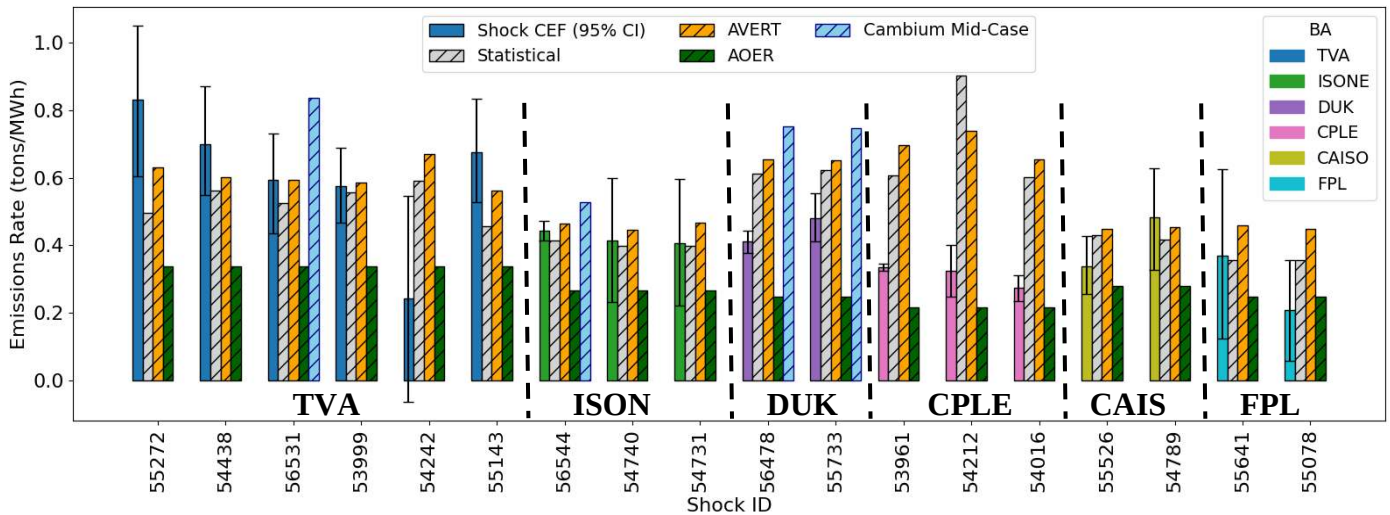
Figure 7: Comparison of the MOER measured using a variety of models against natural experiments from nuclear outages; the model used in this ERS is labelled as “Statistical” (Christian et al., 2025a). Empirically observed emissions rate measured during nuclear outages for each balancing authorities are the left-most solid colored bars for each Shock ID that occurred in each Balancing Authority (BA; 95% confidence interval included), separated by the black dashed-lines: TVA = dark blue bar; ISONE = green bar; DUK = purple bar; CPLE = pink bar; CAISO = yellow bar; and FPL = light blue bar. The hatched bars to the right of each solid bar represent different predicted emissions corresponding to different emissions models : Statistical (MOER) model = grey-hatched bar; AVERT = orange-hatched bar; Cambium Mid-case = light blue-hatched bar; and AOER = green-hatched bar.
