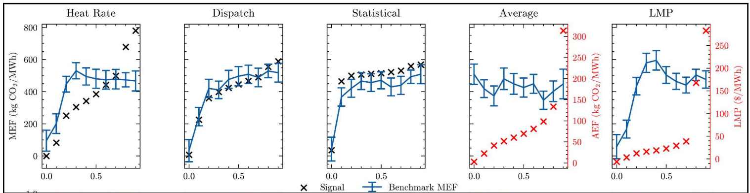
Figure 6: Comparison of the MOER measured using a variety of models against natural experiments from wind generation (top); the model used in this ERS is labelled as “Statistical”, and subplots labelled “Heat Rate”, “Dispatch”, “Average”, and “LMP” are alternative MOER models. The close alignment between the “Statistical” model with the empirical data (“Benchmark MEF”)
