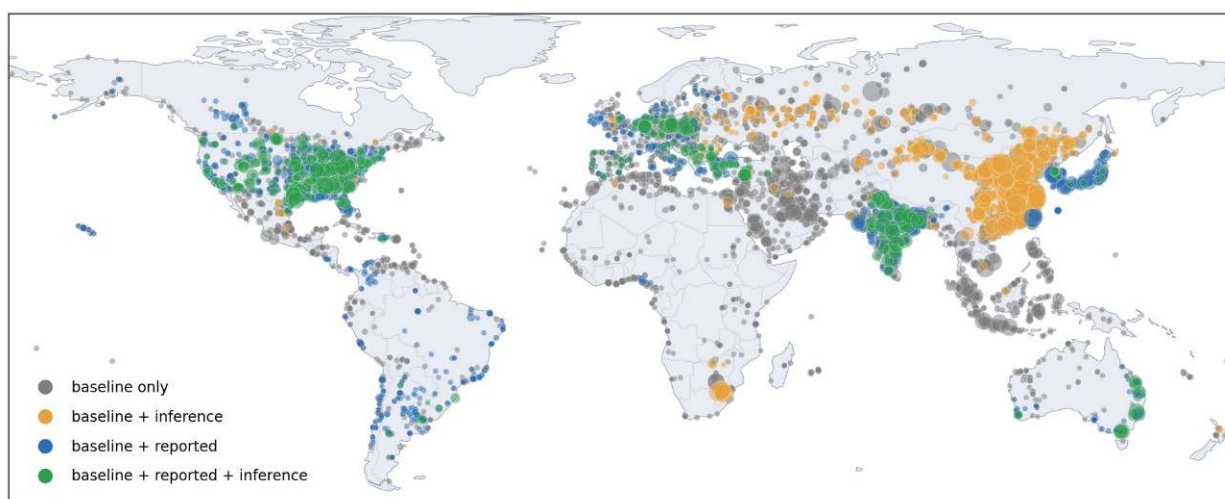
Figure 1: Asset-level Climate TRACE carbon dioxide emissions estimates for January 1, 2025, to December 31, 2025, color-coded by the model types underlying each estimate: emissions based on the baseline country-, and fuel-averages alone (gray), baseline combined with remote sensing inference (yellow), baseline combined with reported data (blue), or baseline combined with both reported data and remote sensing inference (green). Each dot represents one powerplant, sized according to the amount of carbon emissions, ranging from roughly 80 to nearly 33,500,000 metric tons of CO 2 .
