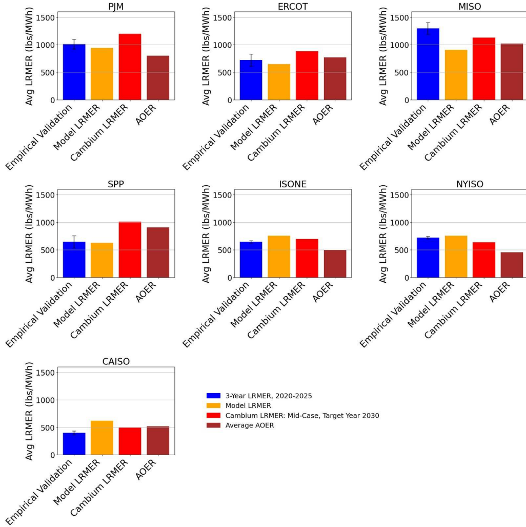
Figure 8: Comparison of the CMER utilized in this ERS (“Model LRMER”) and the empirical validation dataset of the emissions effect of load interventions (“Empirical Validation”). The close agreement between the CMER and the empirical validation signal demonstrates that the CMER reliably captures the real-world emissions impacts of load interventions. Cambium LRMER and AOER refers to other models for computing emissions (see Christian et al., 2025b for details).
