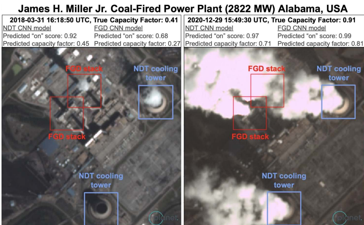
Figure 3: ML predictions on the James H. Miller Jr. power plant at low vs. high generation on two observation dates, using PlanetScope PSScene imagery. Separate natural draft cooling tower (NDT) and flue gas desulfurization (FGD) models predicted on NDT (blue) and FGD stacks (red) patches. These predictions were ingested by subsequent models to estimate generation, then CO 2 , SO 2 , NO x , and PM 2.5 , for the plant. © 2023 IEEE [8].
